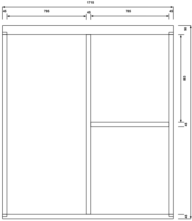
FRONT WALL
